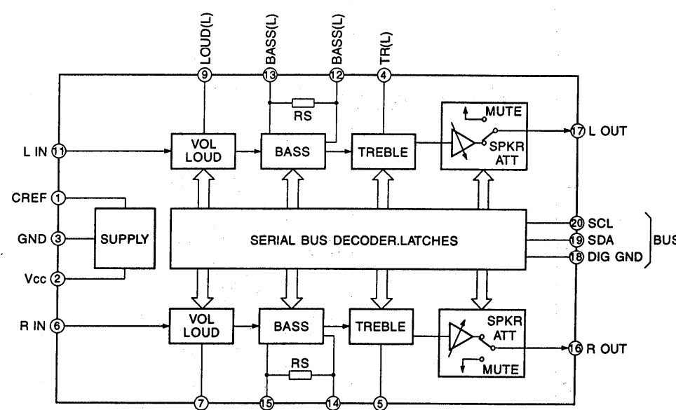
U BOARD IC1141 TDA7315
