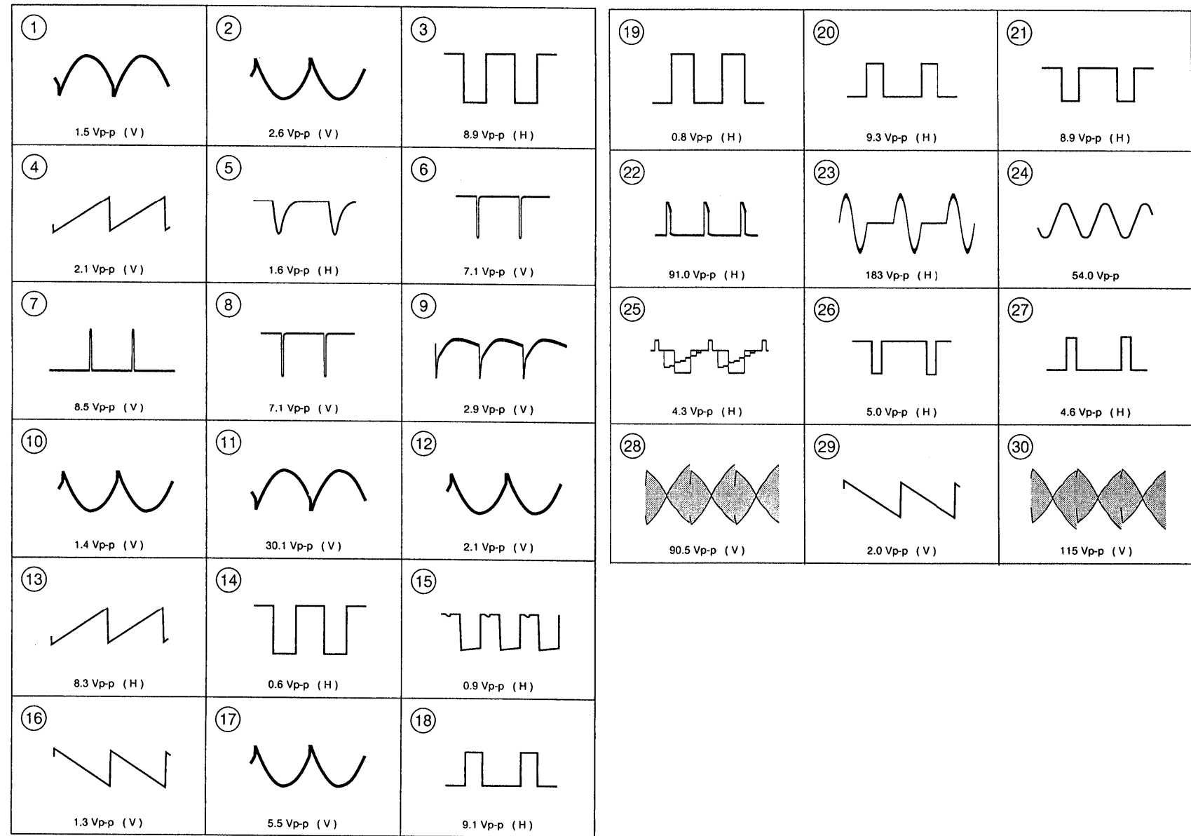
D BOARD WAVEFORMS
