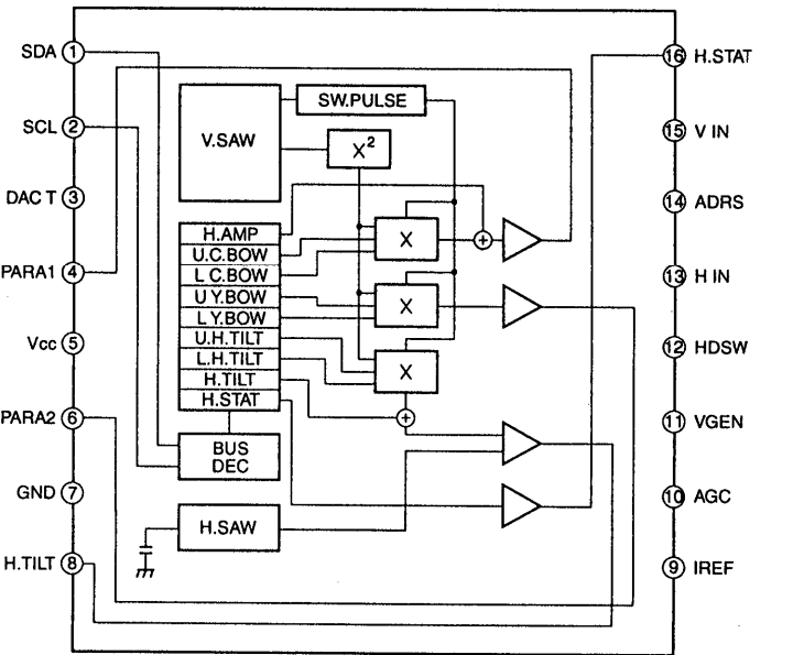
D BOARD IC802 CXA1526P
